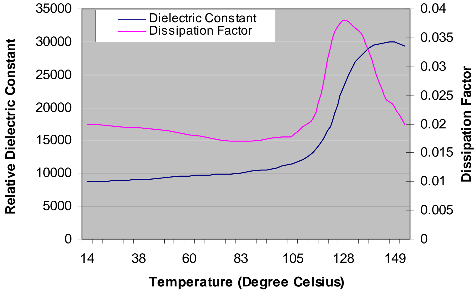
DL-61HD Temperature Dependence of Dielectric Properties
