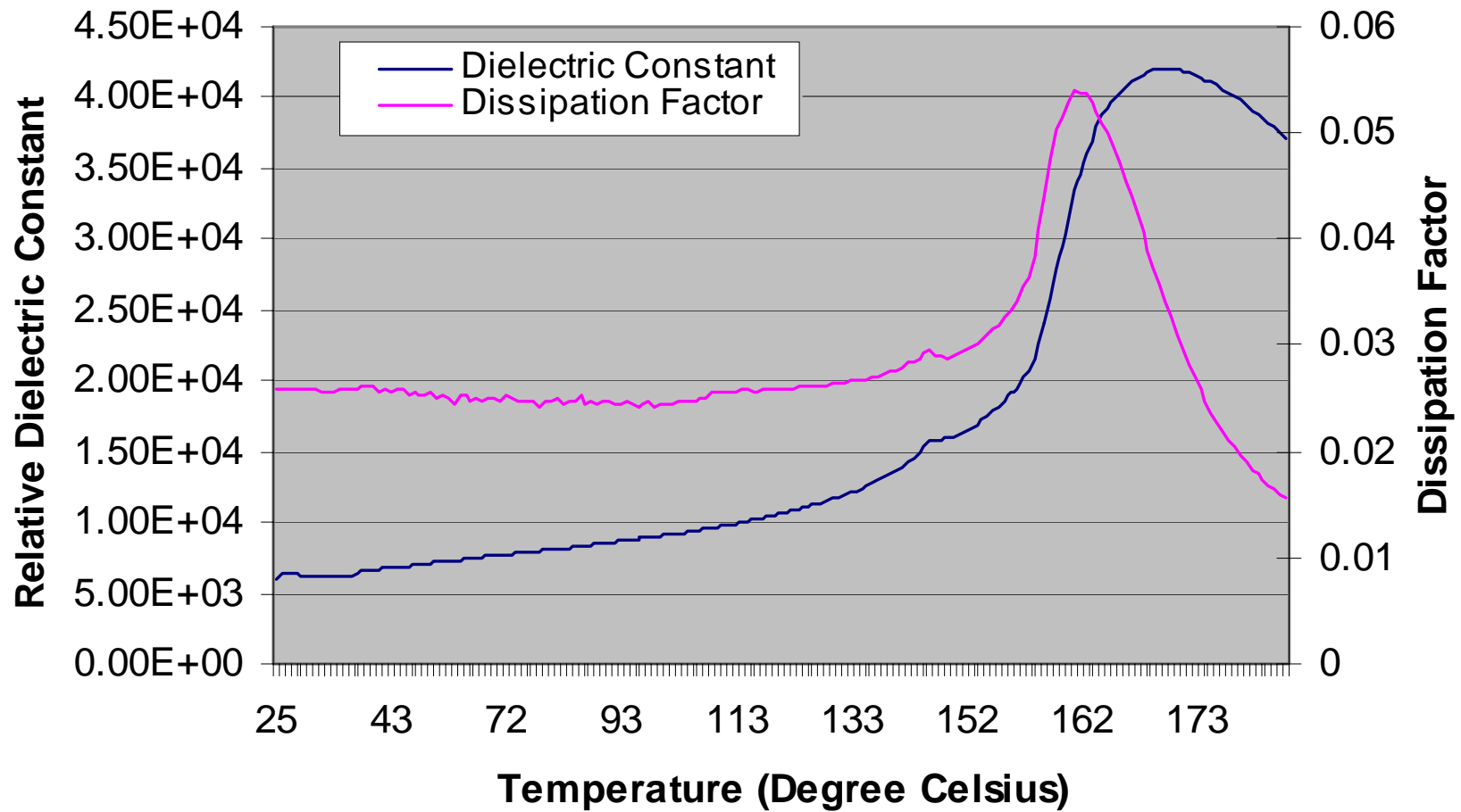
DL-60HD Temperature Dependence of Dielectric Properties
