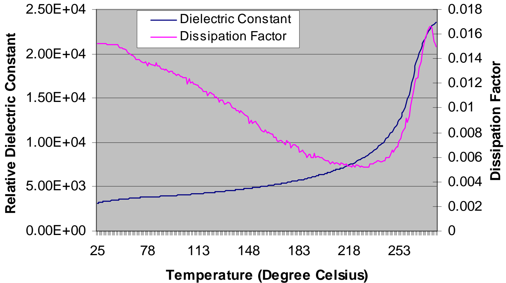
DL-52HD Temperature Dependence of Dielectric Properties
