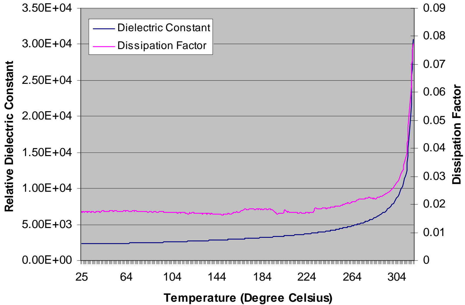
DL-51 Temperature Dependence of Dielectric Properties
