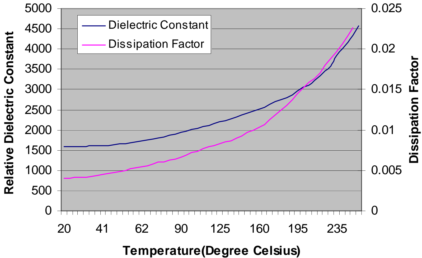
DL-47 Temperature Dependence of Dielectric Properties
