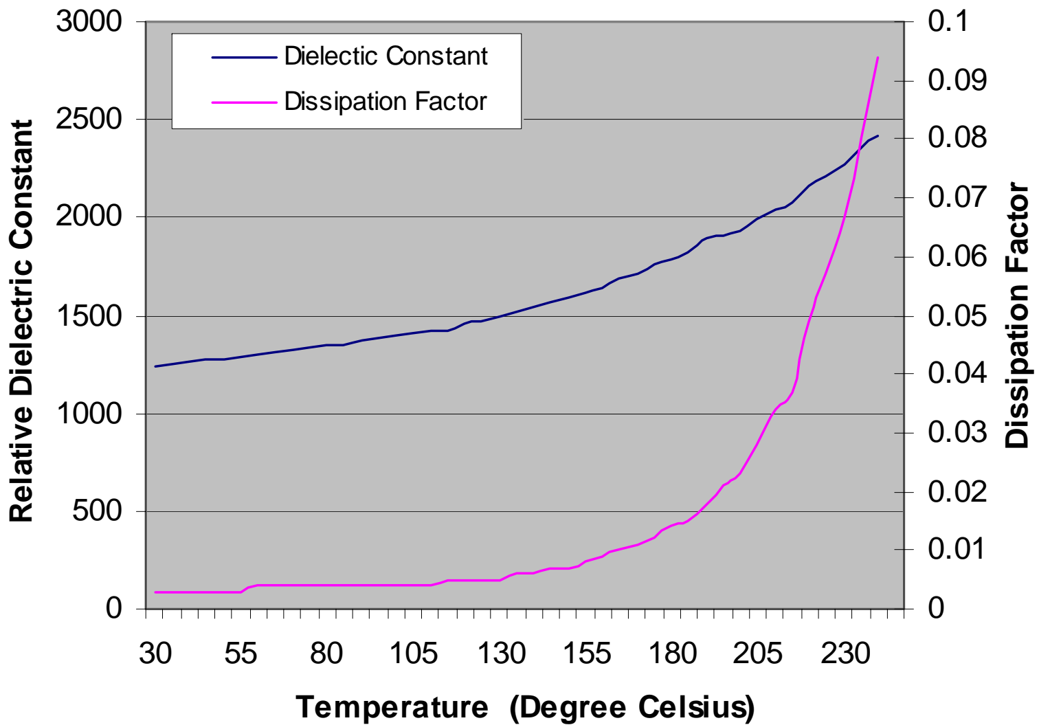
DL-45 Temperature Dependence of Dielectric Properties
