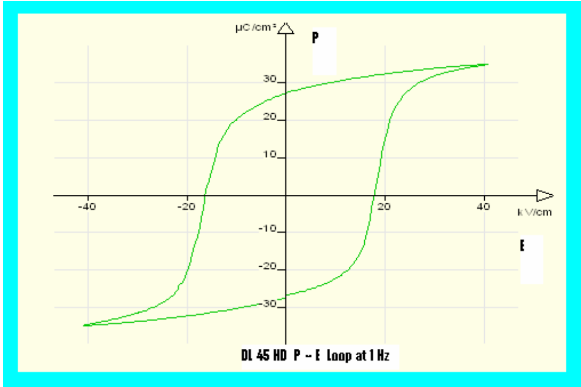
DL-45HD P-E LOOP
