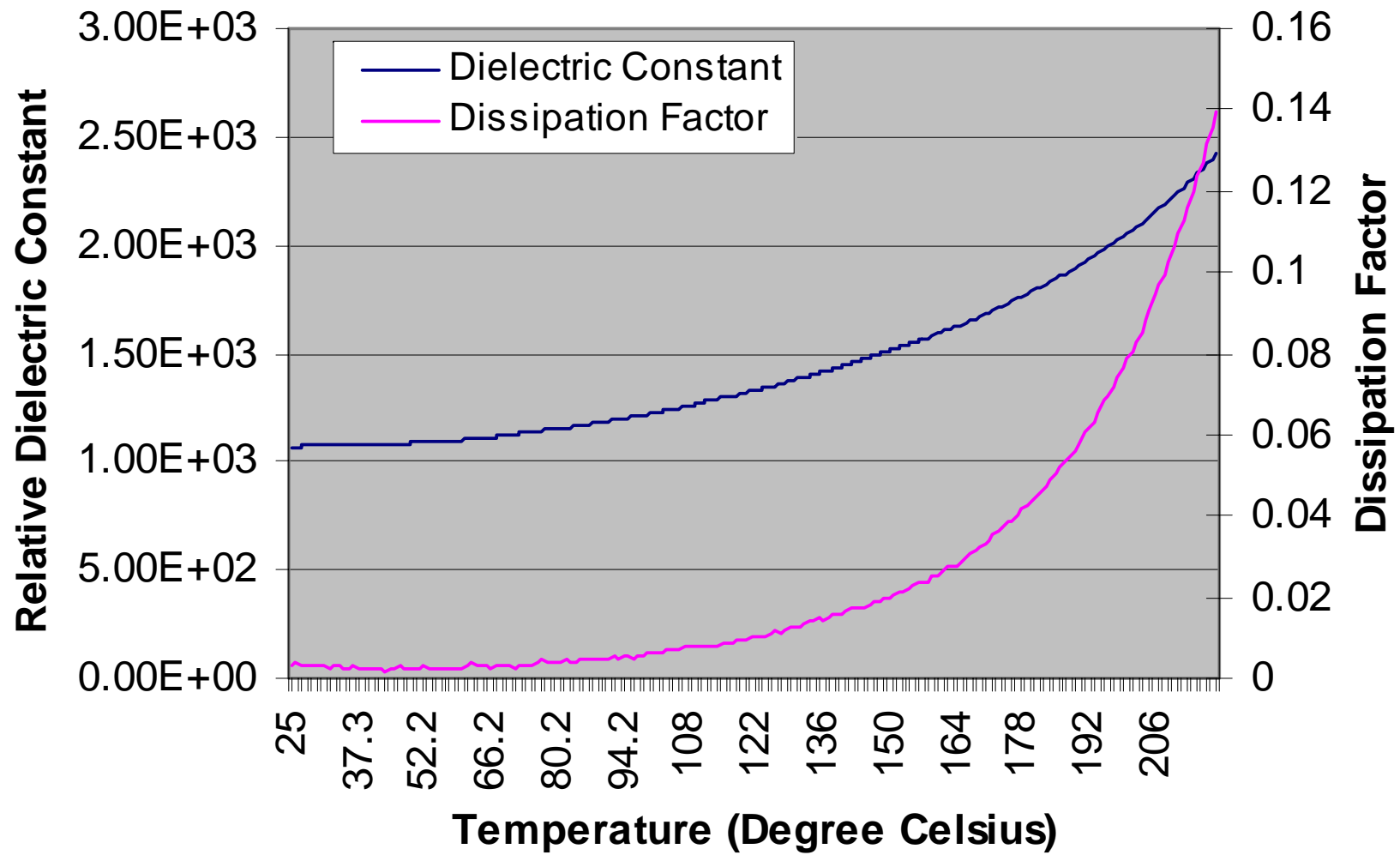
DL-43 Temperature Dependence of Dielectric Properties
