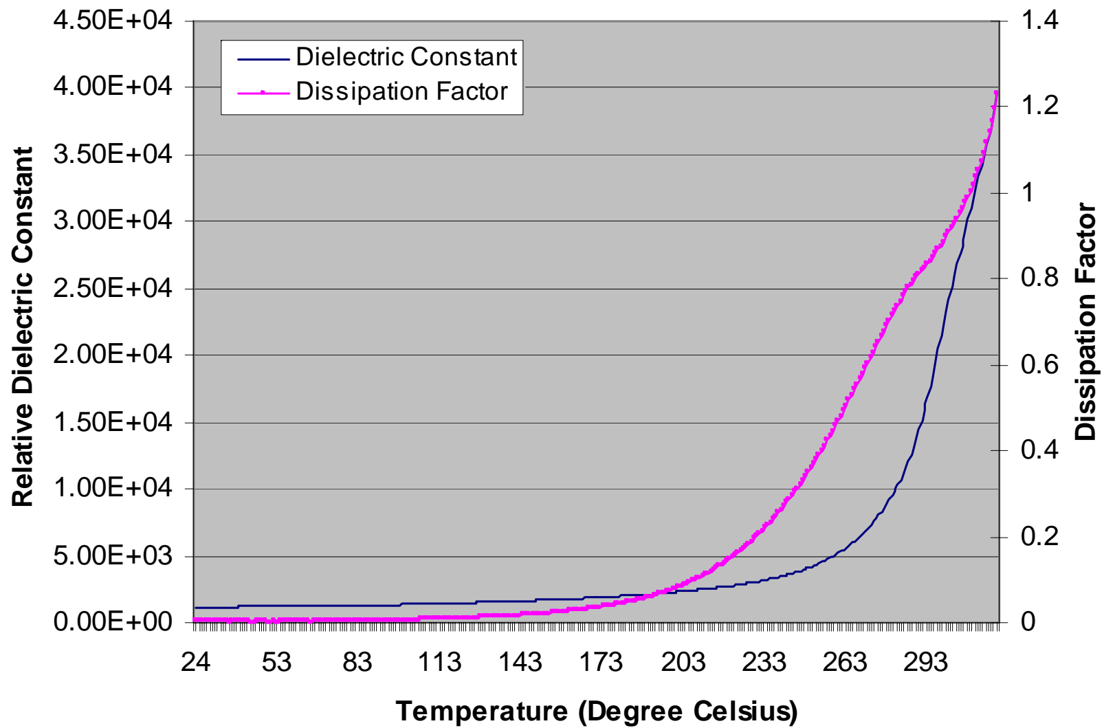
DL-43HD Temperature Dependence of Dielectric Properties
