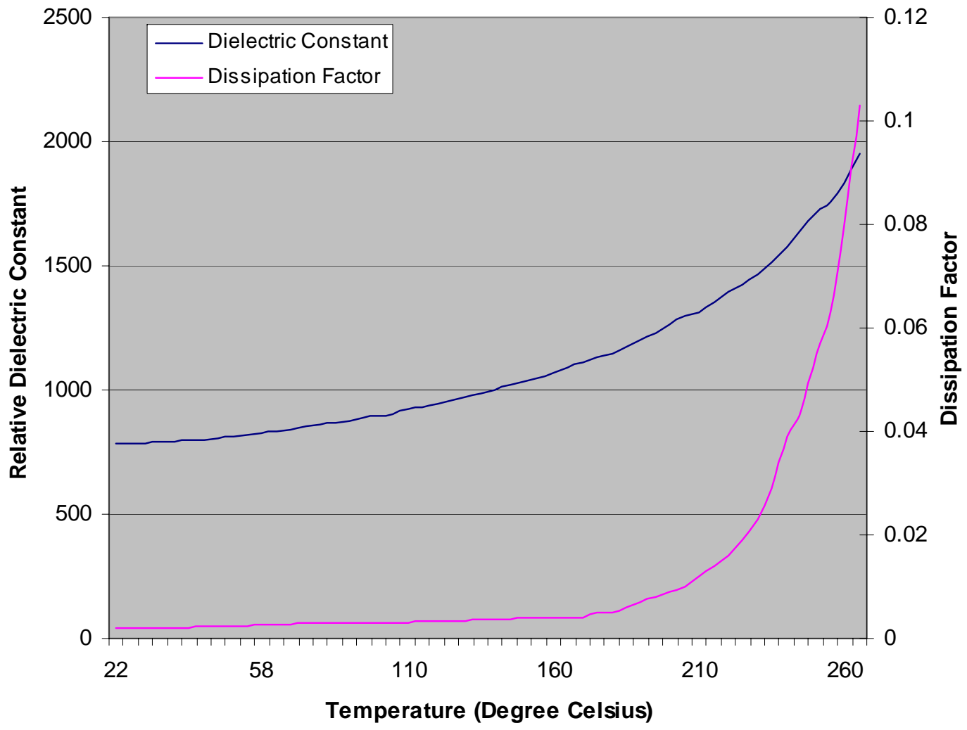
DL-42 Temperature Dependence of Dielectric Properties
