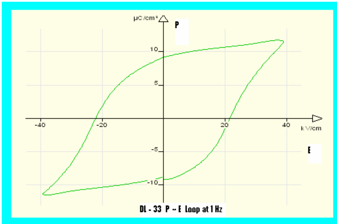
DL-33 P-E LOOP
