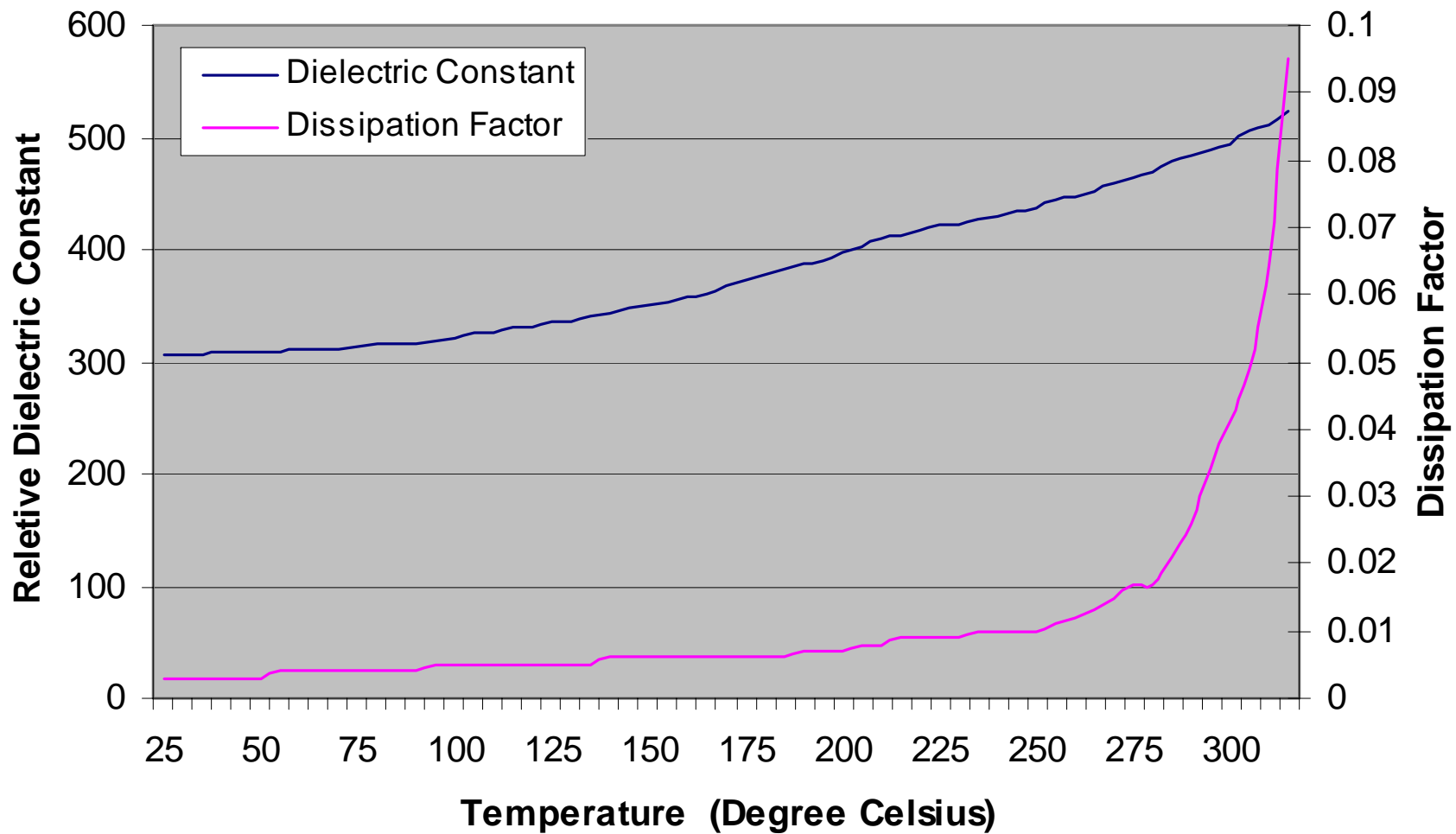
DL-31 Temperature Dependence of Dielectric Properties
