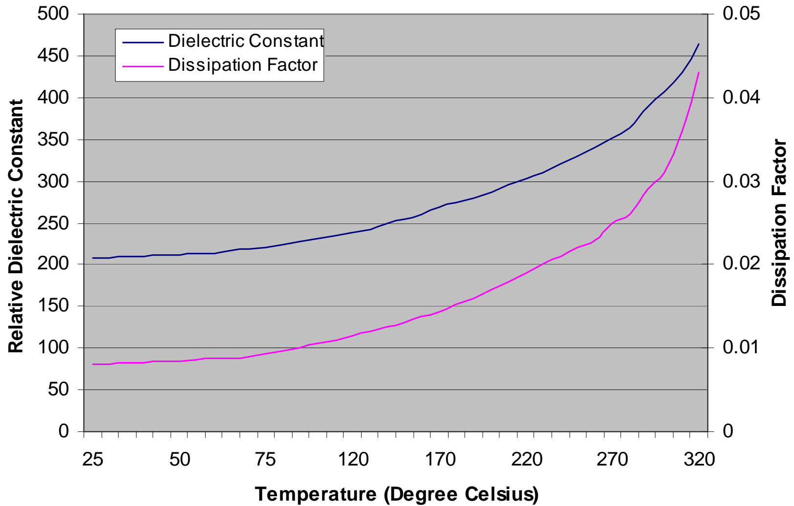
DL-20 Temperature Dependence of Dielectric Properties
