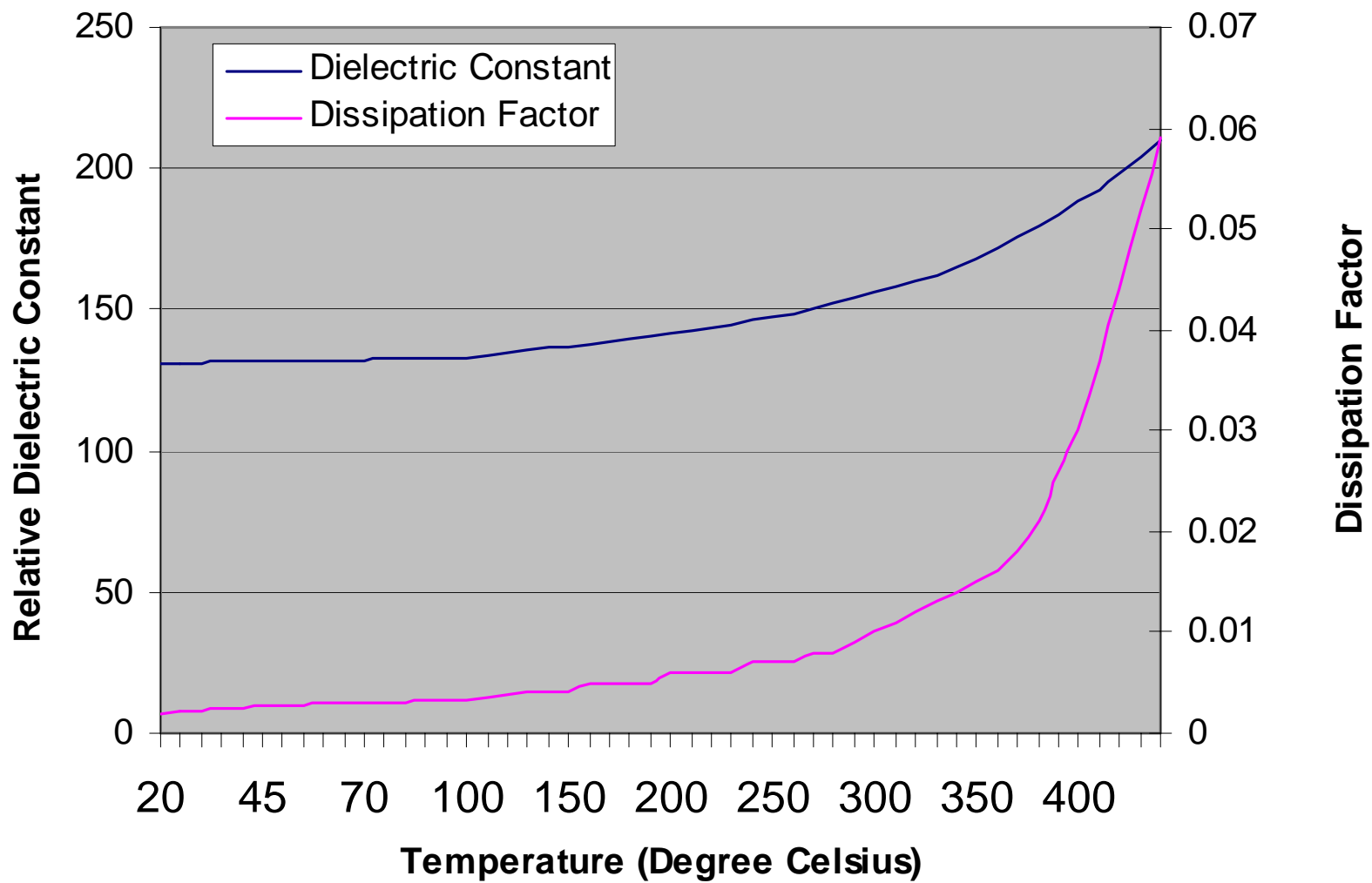
DL-10 Temperature Dependence of Dielectric Properties
