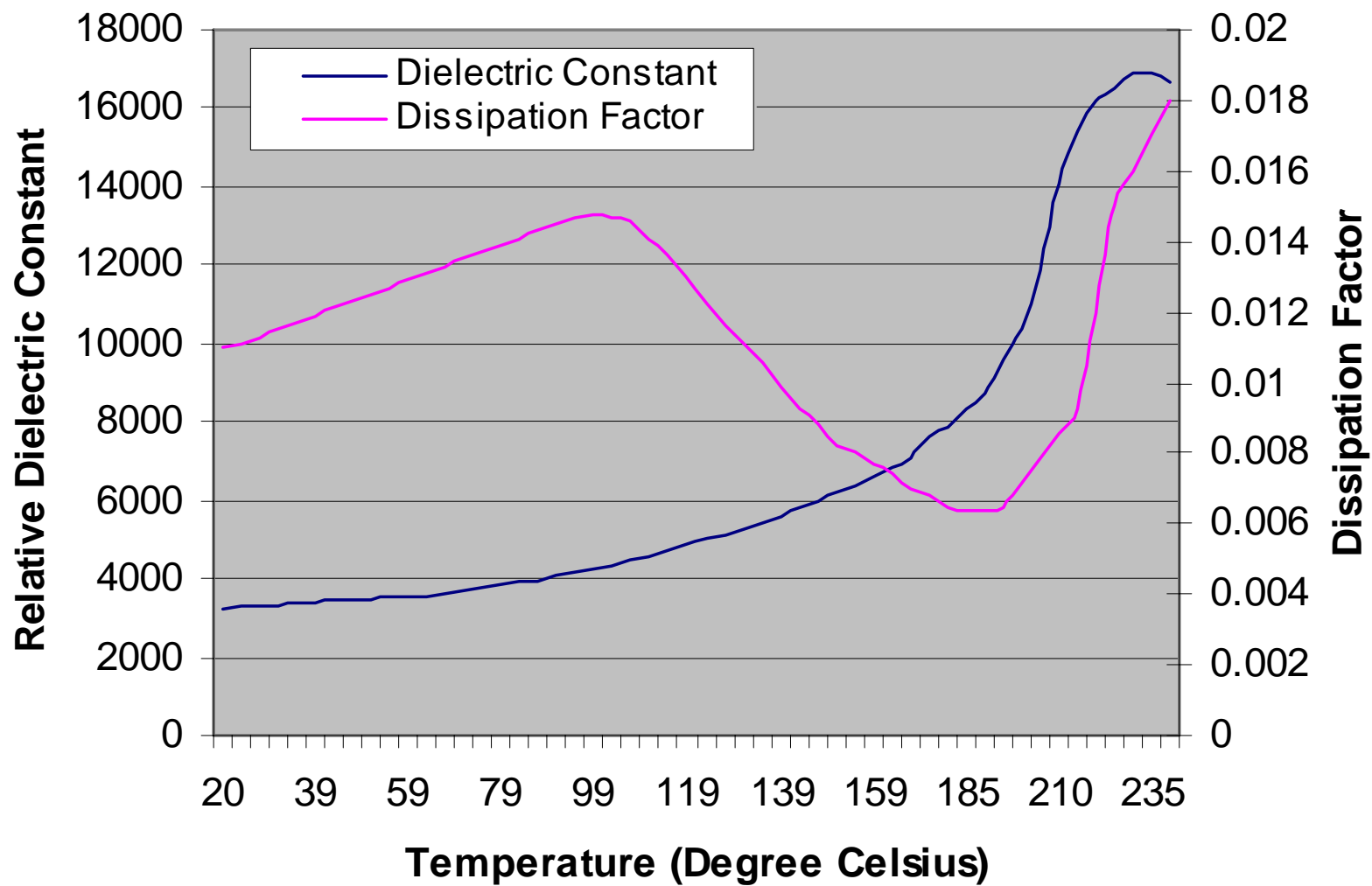
DL-53 Temperature Dependence of Dielectric Properties
