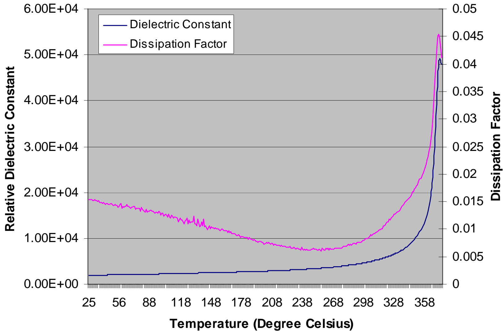
DL-50HD Temperature Dependence of Dielectric Properties
