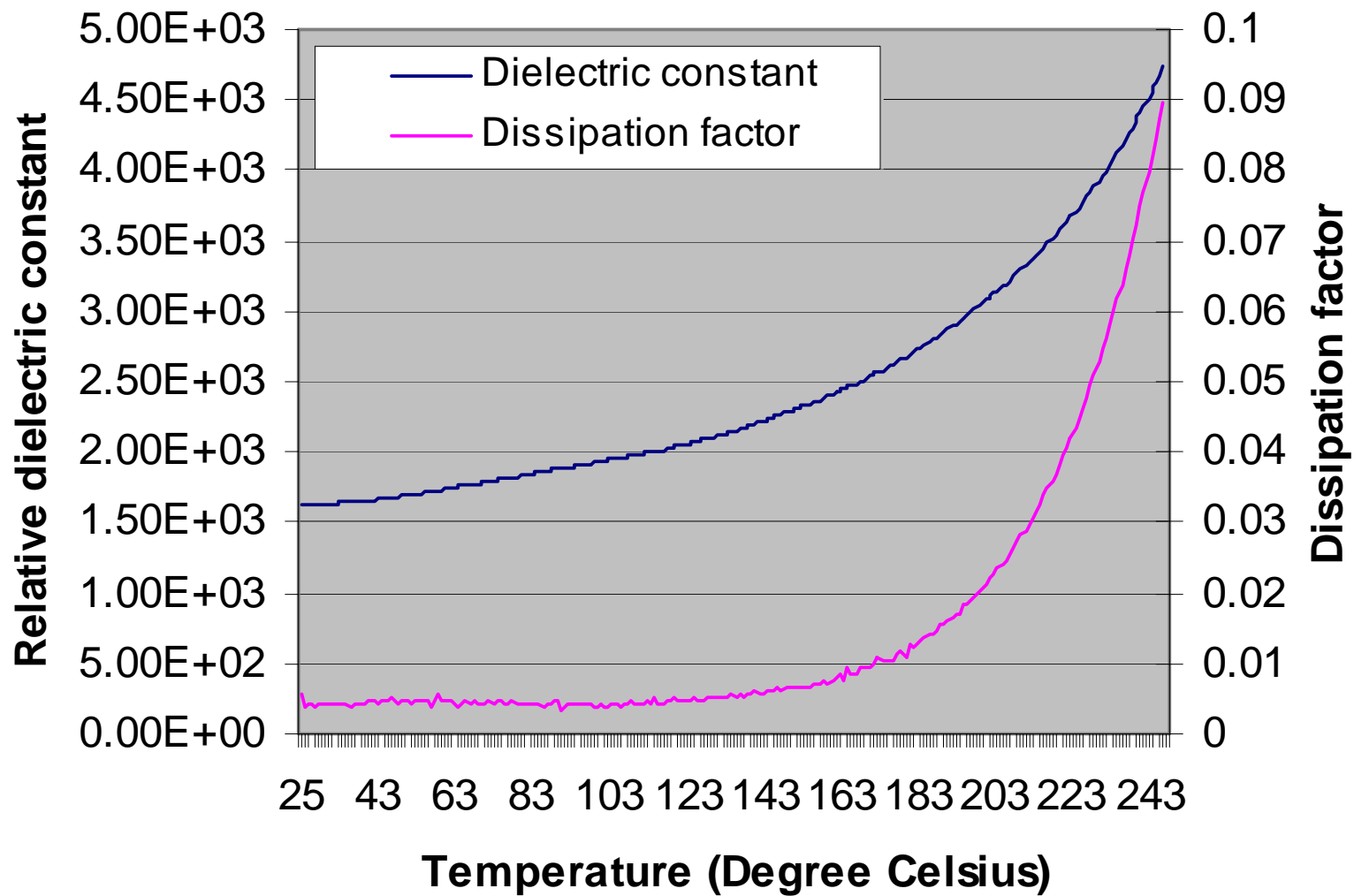
DL-45HD Temperature Dependence of Dielectric Properties
