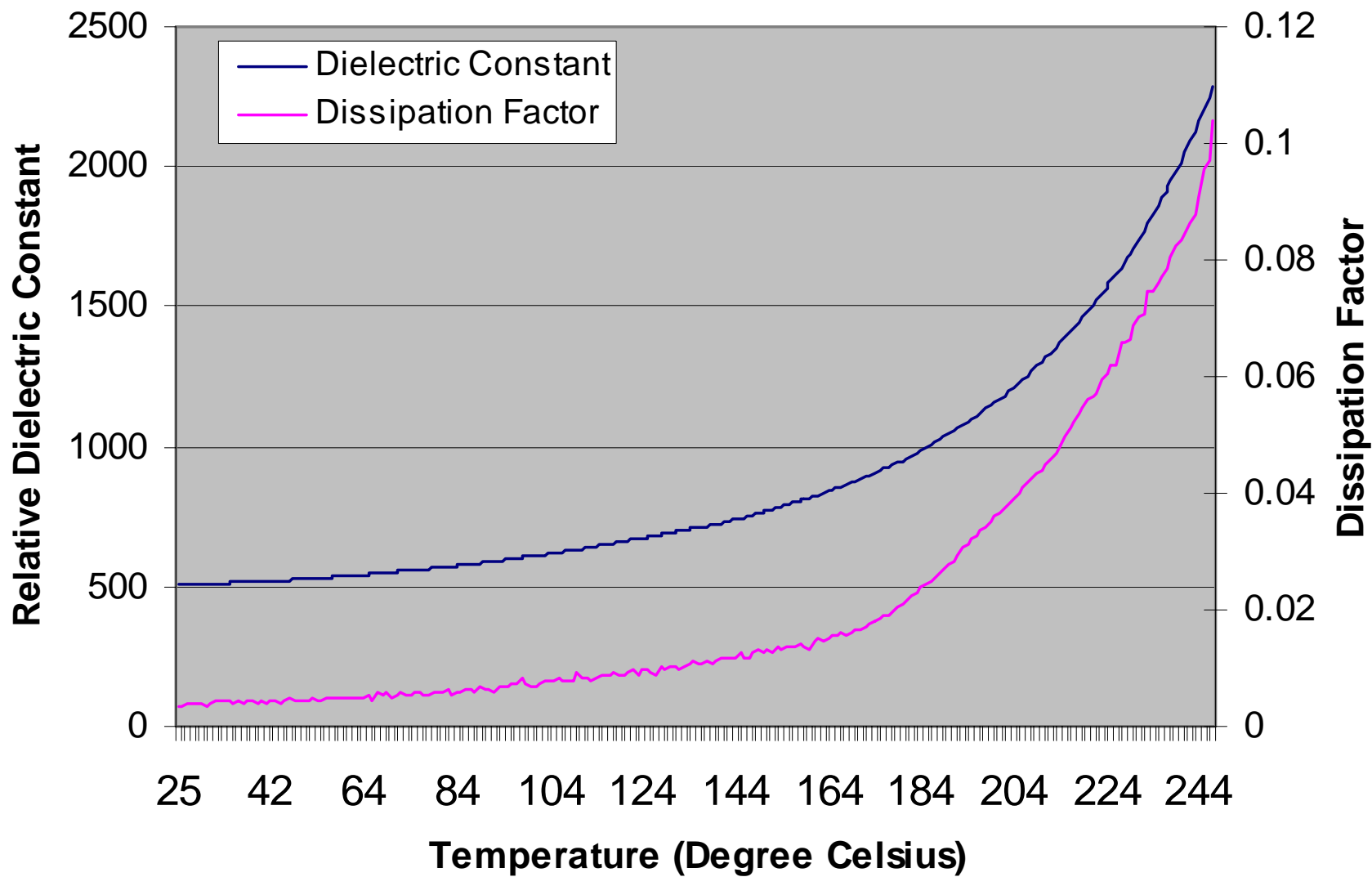
DL-41 Temperature Dependence of Dielectric Properties
