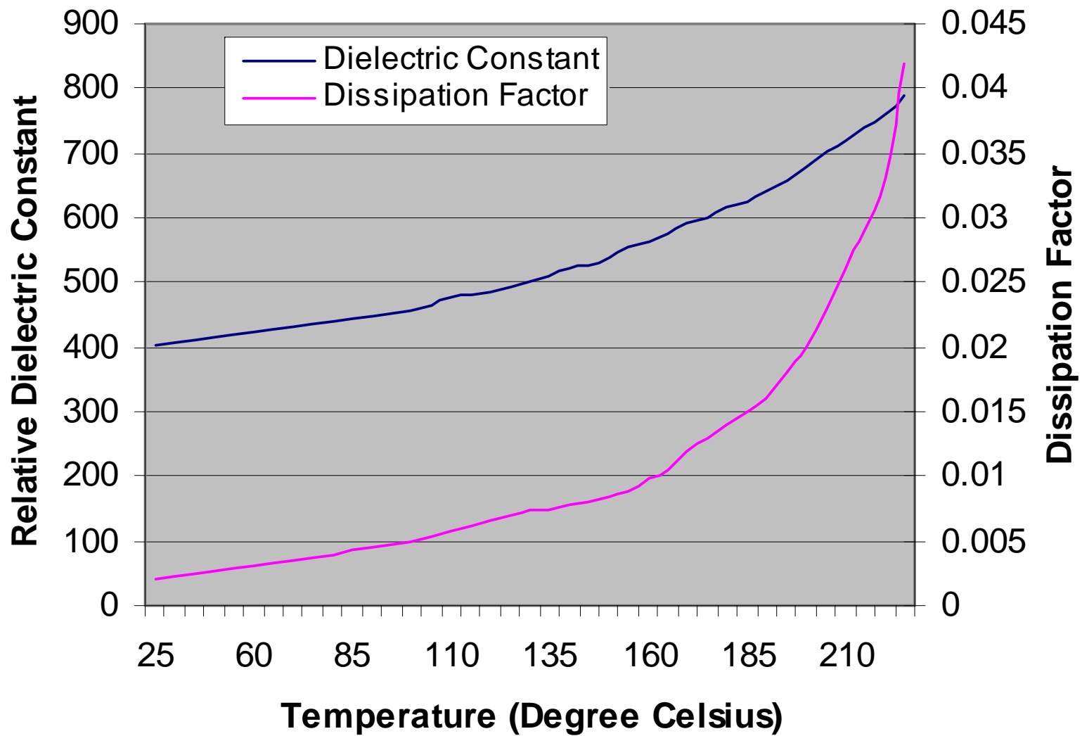
DL-40 Temperature Dependence of Dielectric Properties
