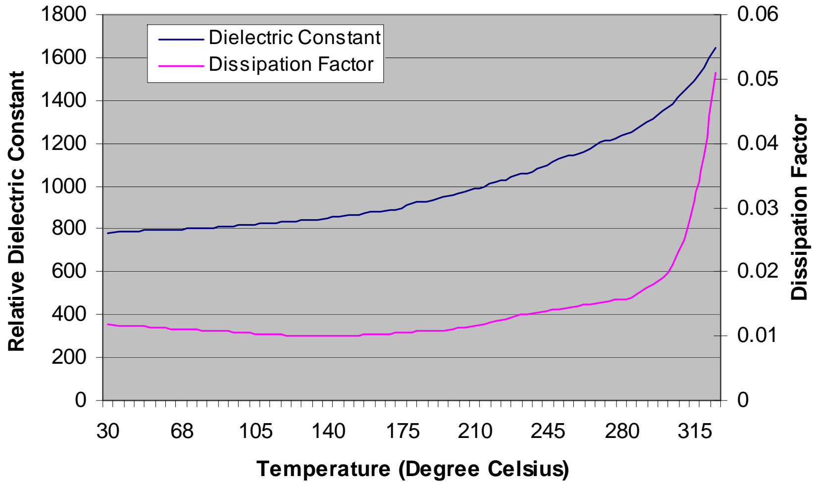
DL-32 Temperature Dependence of Dielectric Properties
